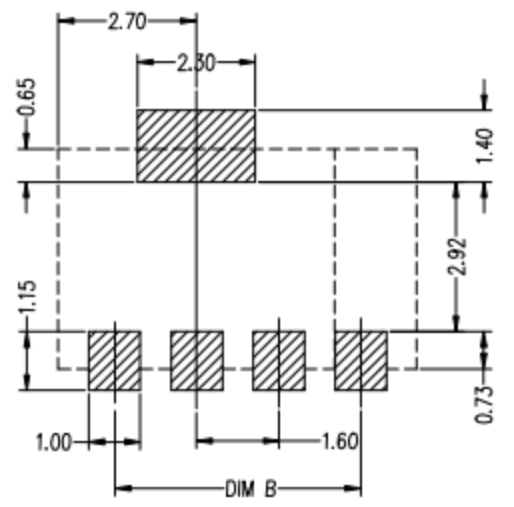
RECOMMENDED PCB LAYOUT TDL:(±0.05)
