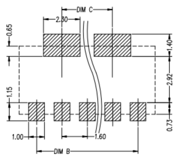
RECOMMENDED PCB LAYOUT TDL:(±0.05)
